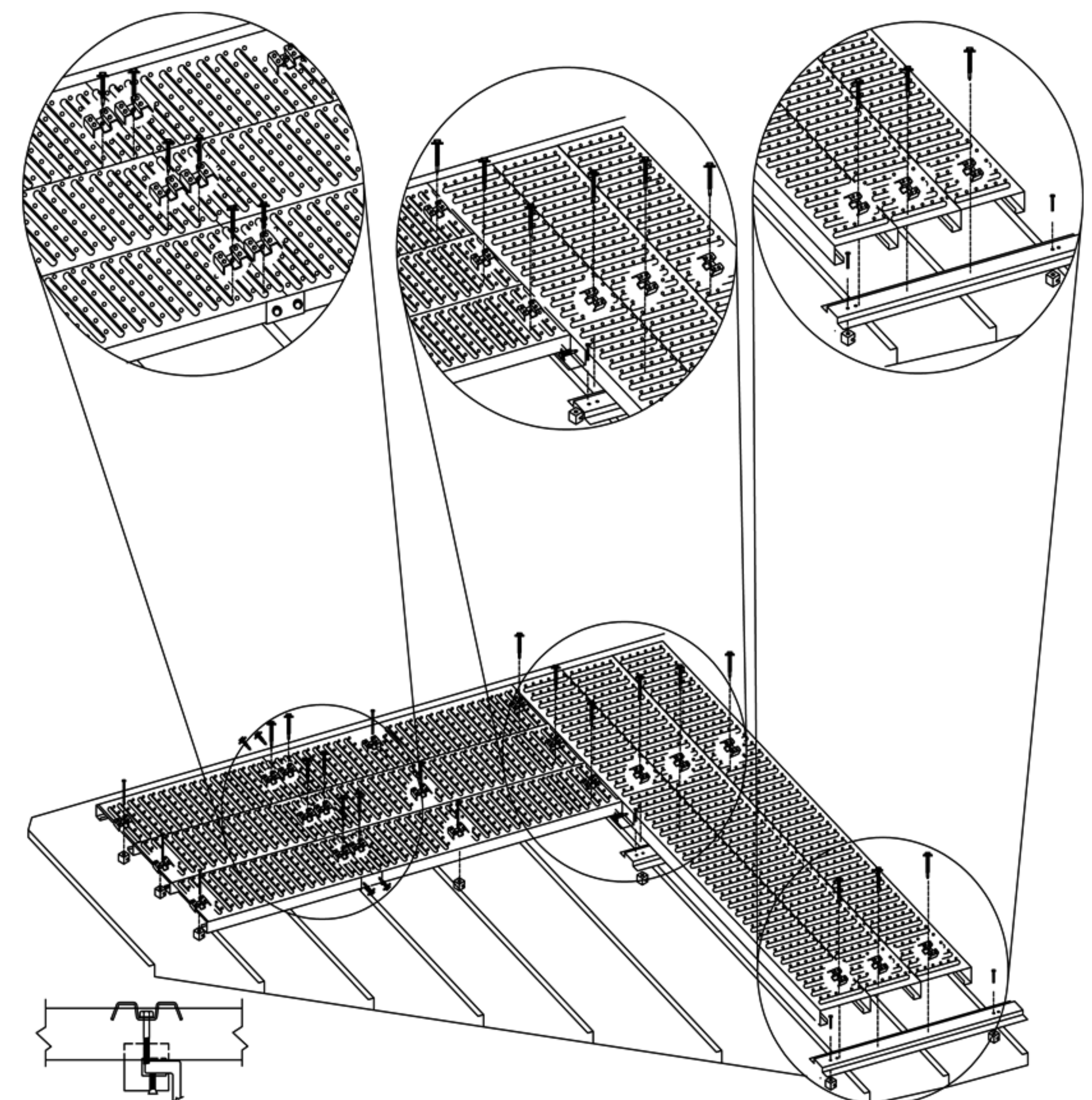
RW36 BATTEN STANDING SEAM
